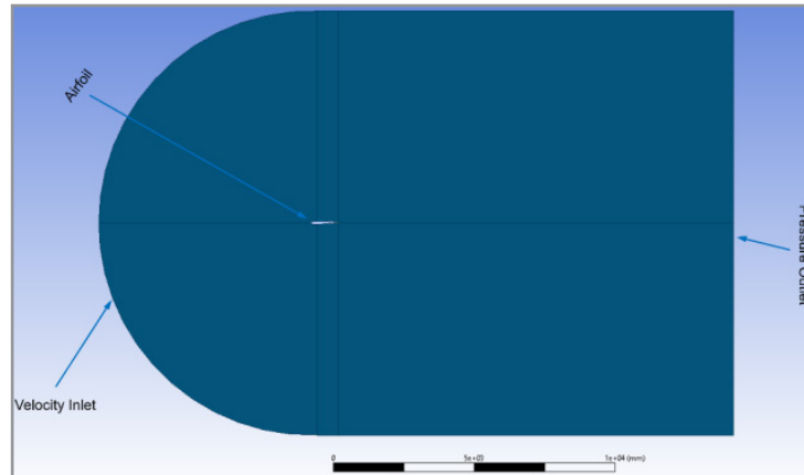
Figure 1: Computational domain and boundary extents around the airfoil.
