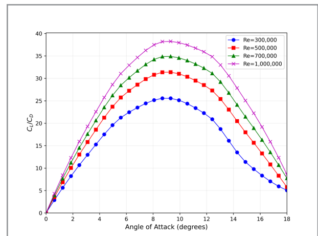
Figure 18: C_L/C_D Vs AOA for NACA 0020 Profiles at different Reynolds Numbers
